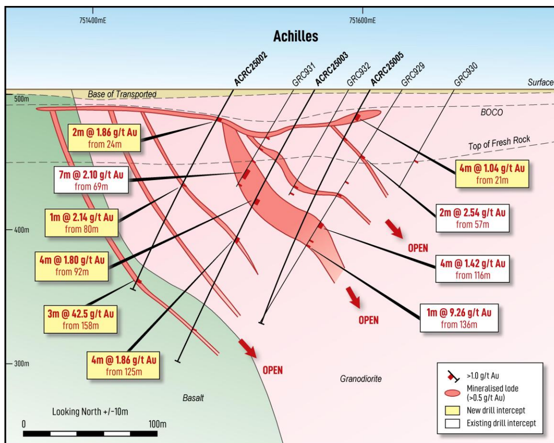
Figure 5: Cross section A-A' at the Achilles North Deposit
