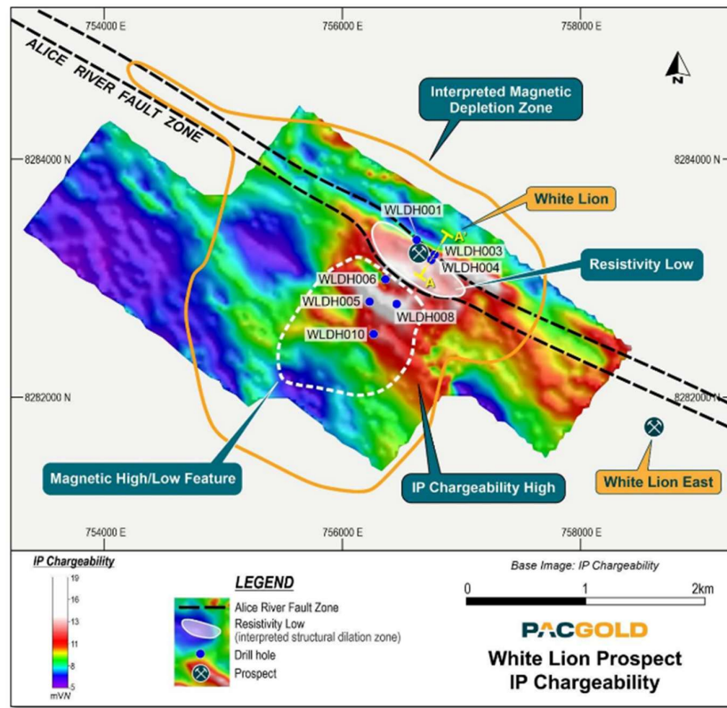
Figure 11: White Lion Prospect RC drillhole location on IP Chargeability
