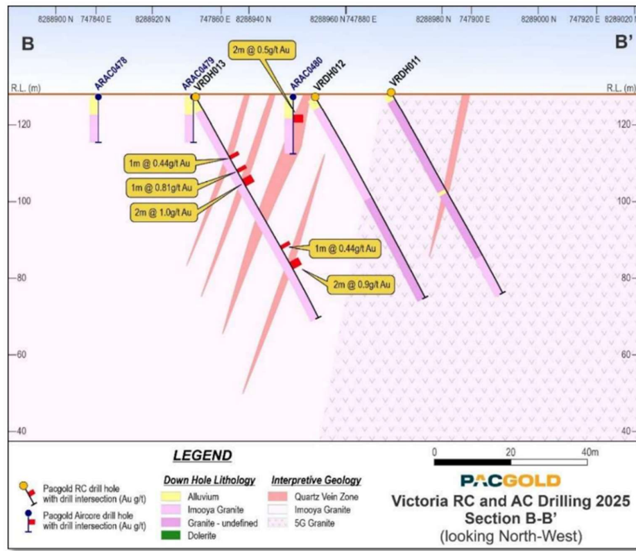
Figure 10: Victoria RC Drilling section B – B'
