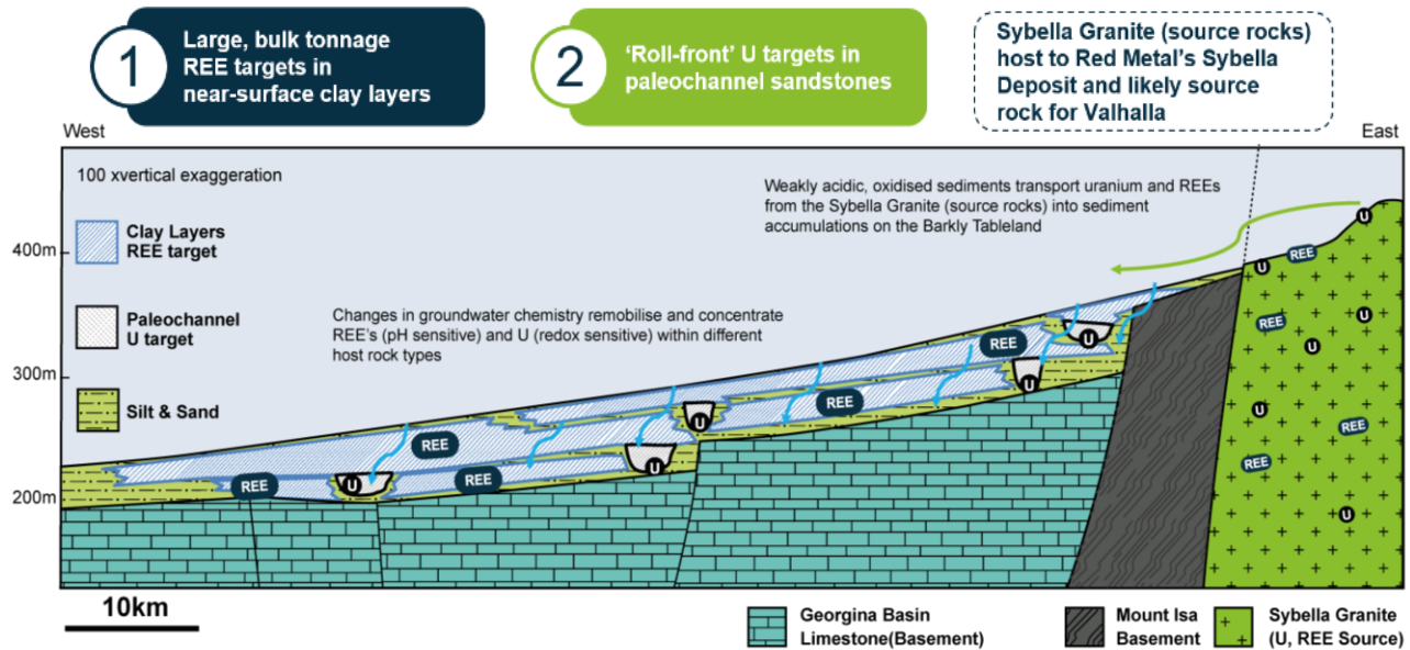
Figure 3 – Schematic cross-section of sediment-hosted mineralisation models
