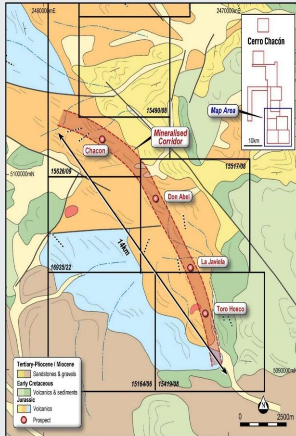
Figure 1: Cerro Chacon 14km mineralised corridor - ~8500m RC drilling scheduled to commence in October
