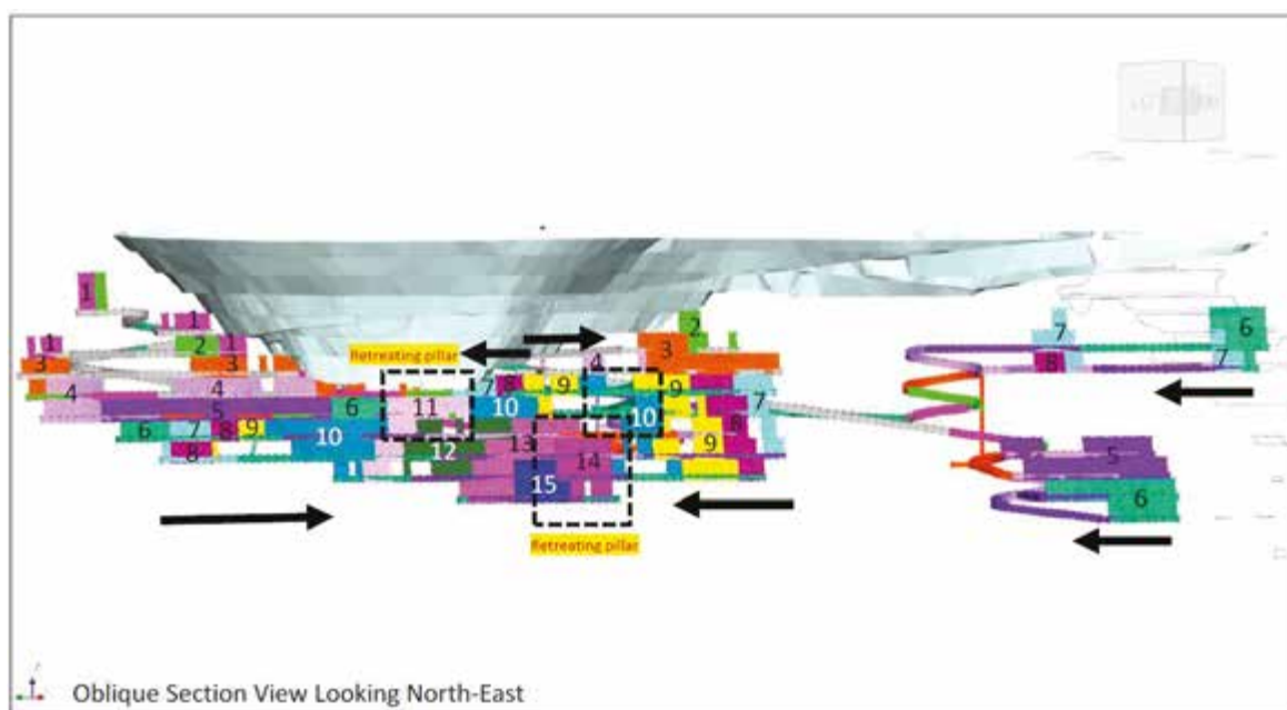
Figure 6.5: Yunndaga underground mine design with mining sequence
