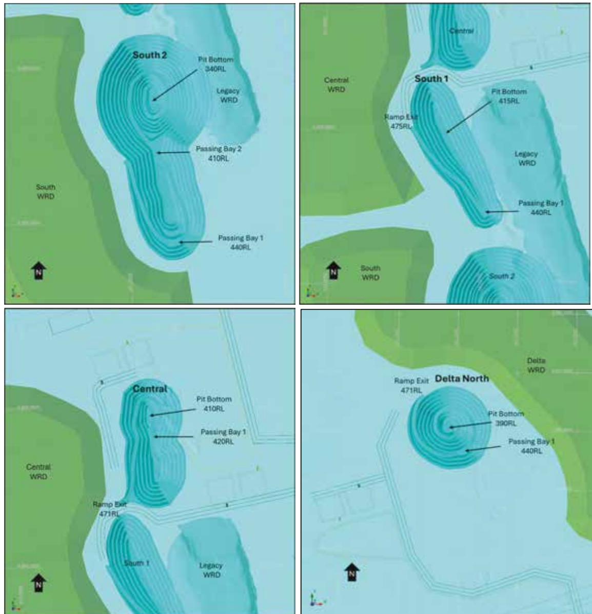
Figure 5.9: Cork Tree Well pit designs – South 1, South 2, Central and Delta North
