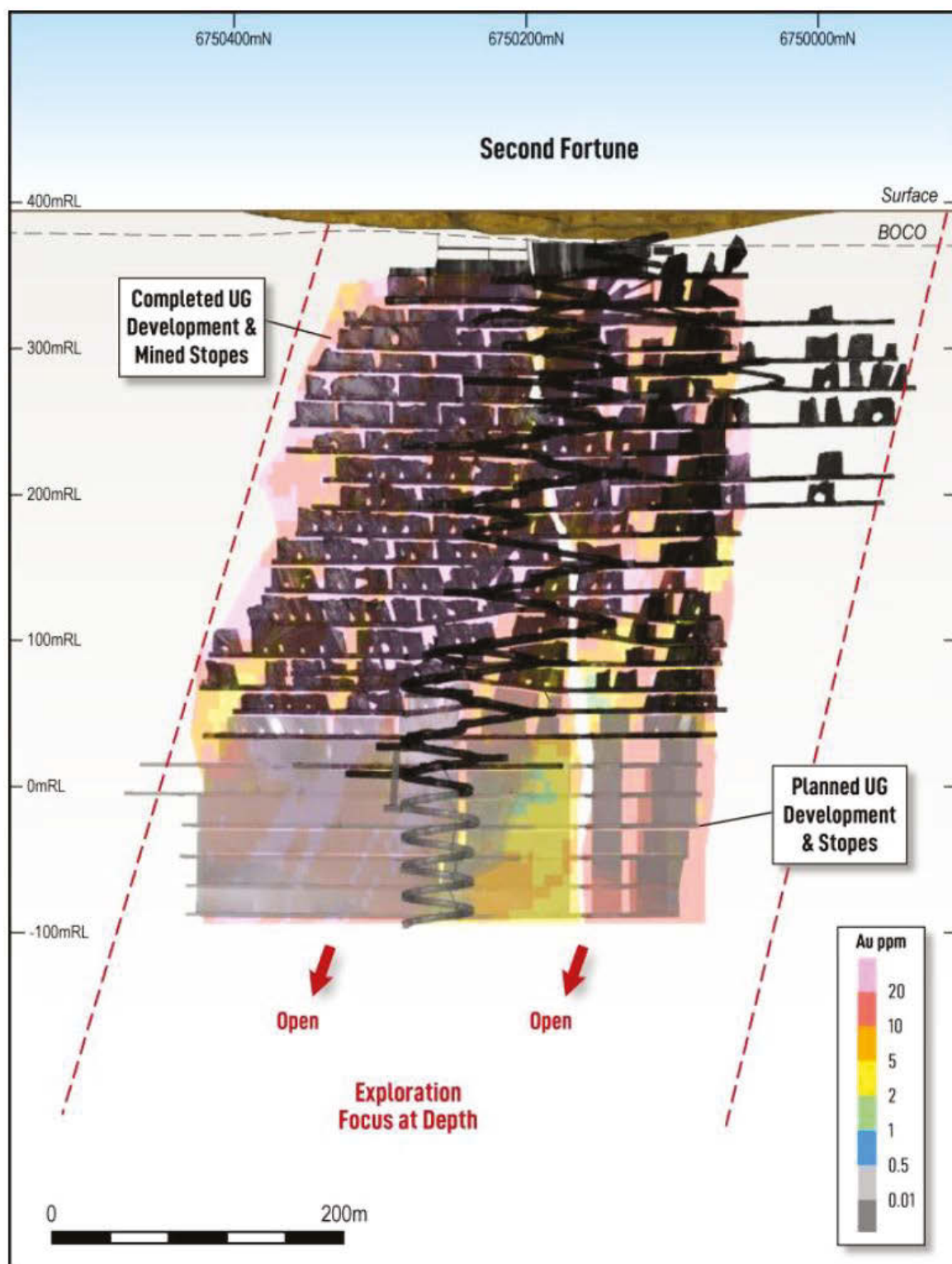
Figure 5.11: Second Fortune mine long-section – 2025 MRE
