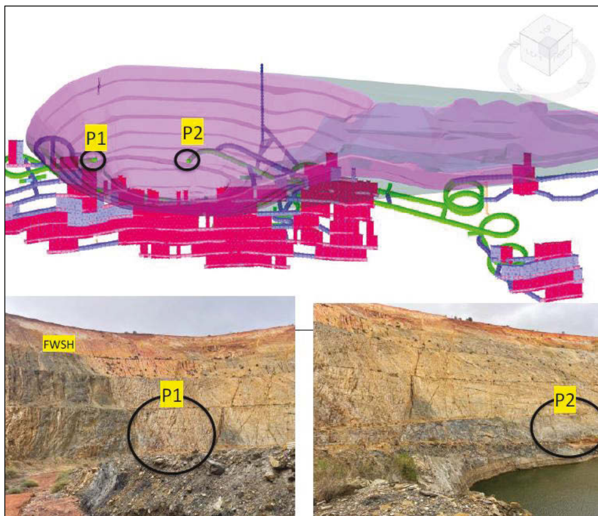
Figure 6.6: Proposed portal locations in the existing Yunnadaga pit
