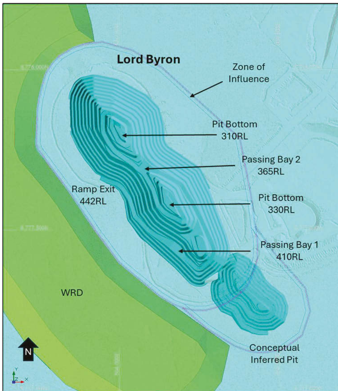
Figure 5.8: Lord Byron pit design
