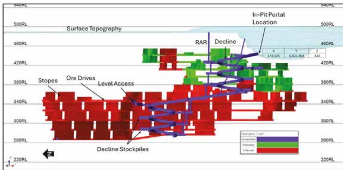
Figure 5.13: Alpha underground mine design with Mineral Resource classes
