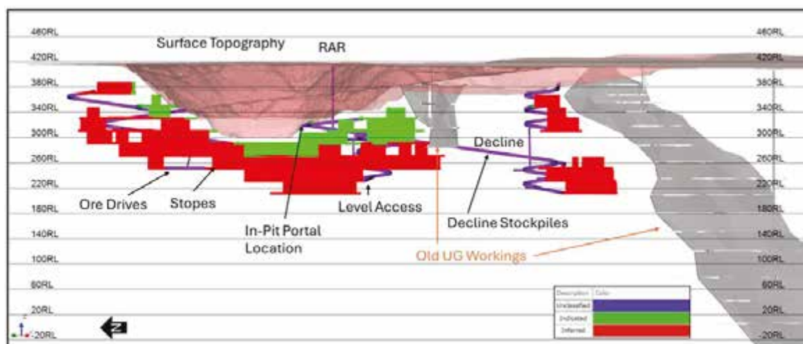
Figure 6.4: Yunndaga historical workings and scoping study mine design
