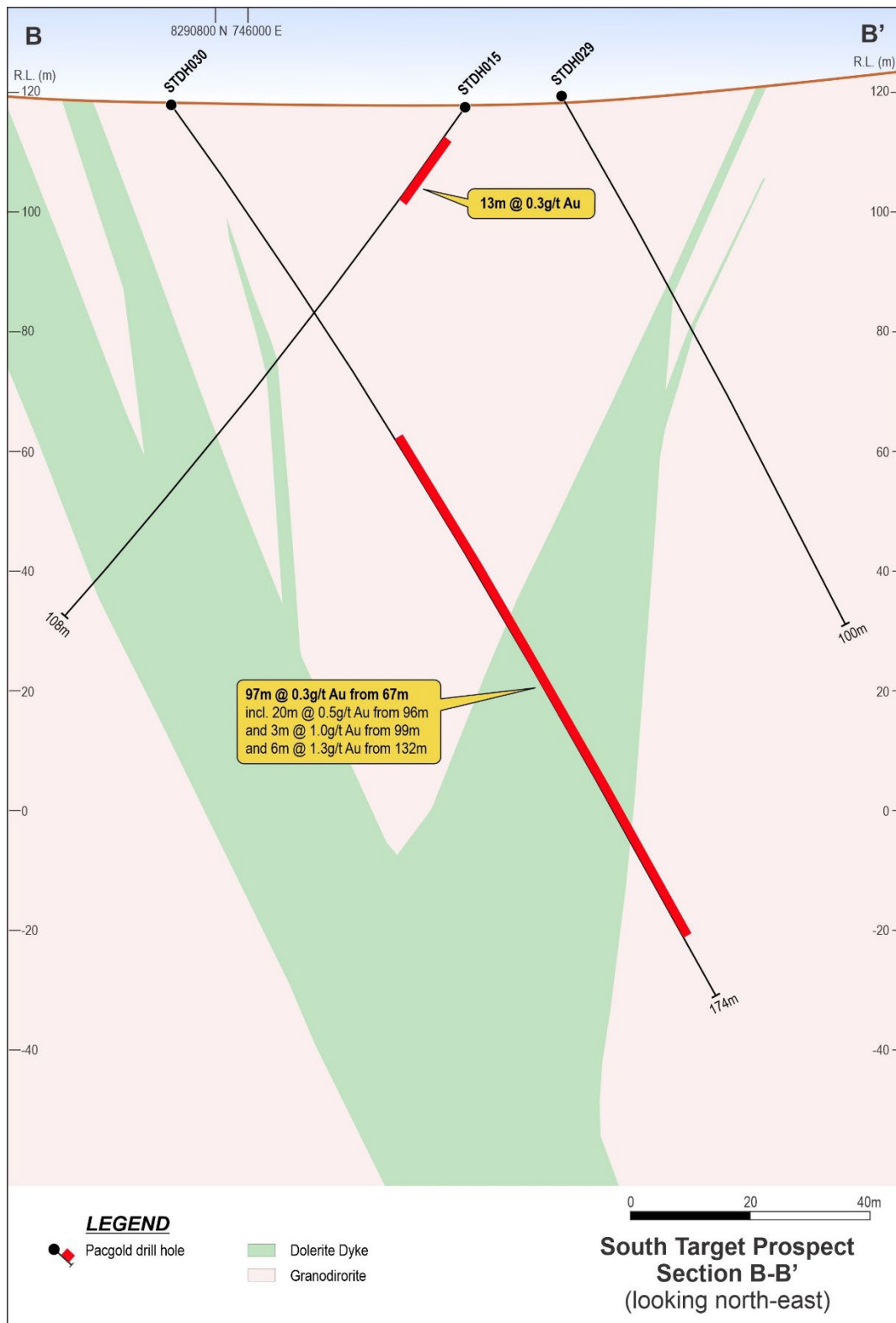
Figure 2: Section B-B' through Southern Target area with historic and new drilling
