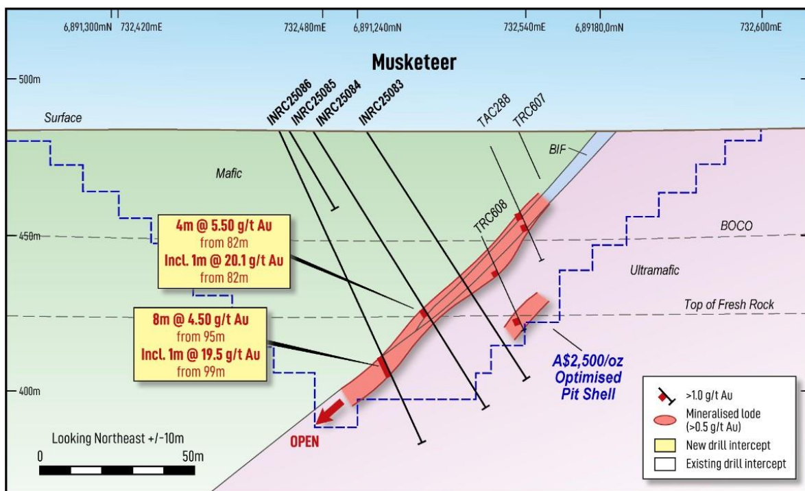
Figure 5 - Musketeer Cross-section A-A'
