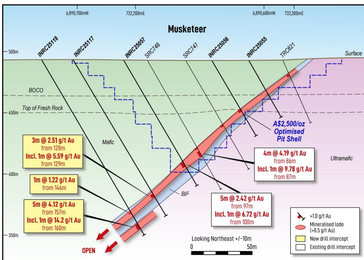
Figure 6 - Musketeer Cross-section B-B'
