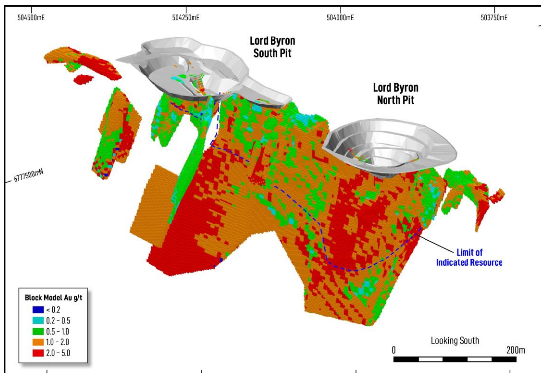
Figure 2: The 2025 Lord Byron MRE, coloured by grade. Note: unclassified areas of the model are not shown on this image. Only reported resource categories (Measured, Indicated, and Inferred) are shown
