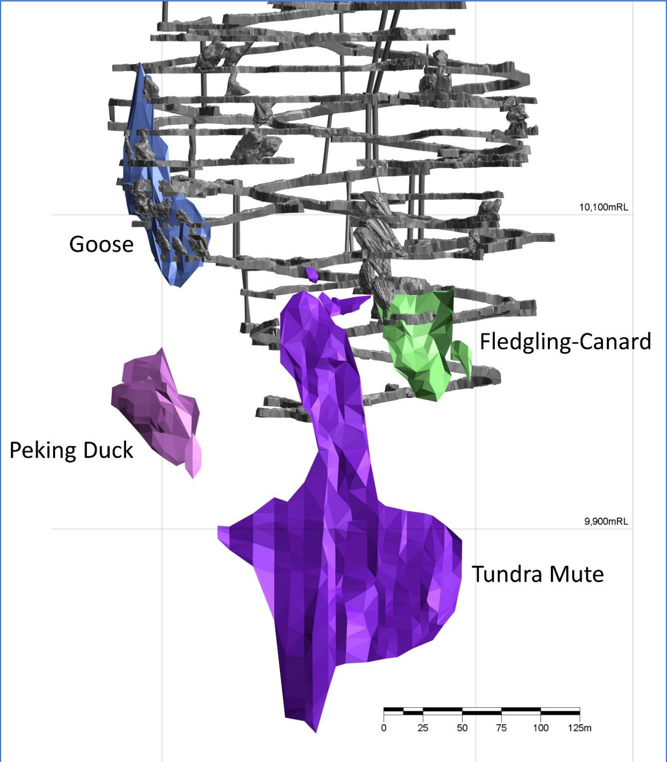
Figure 3: Long section looking West showing simplified layout of the Silver Swan Deposits.
