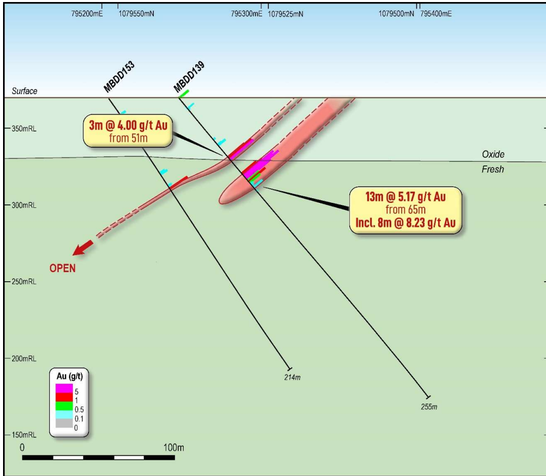
Figure 4: Oblique Cross Section looking northeast (+/-50m) showing new drill results MBDD139 – BM Target 3
