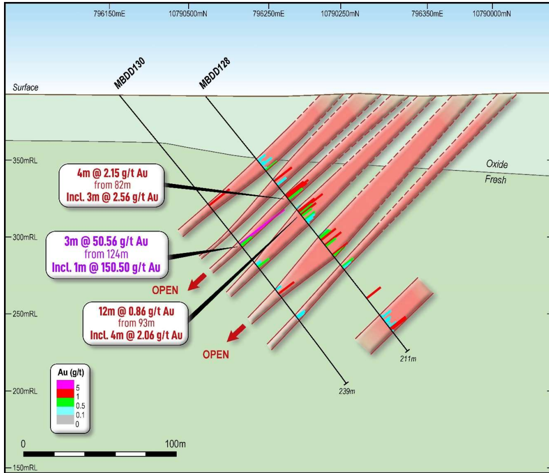
Figure 4: Oblique Cross Section looking northeast (+/-50m) showing new drill results MBDD130 – BM Target 3
