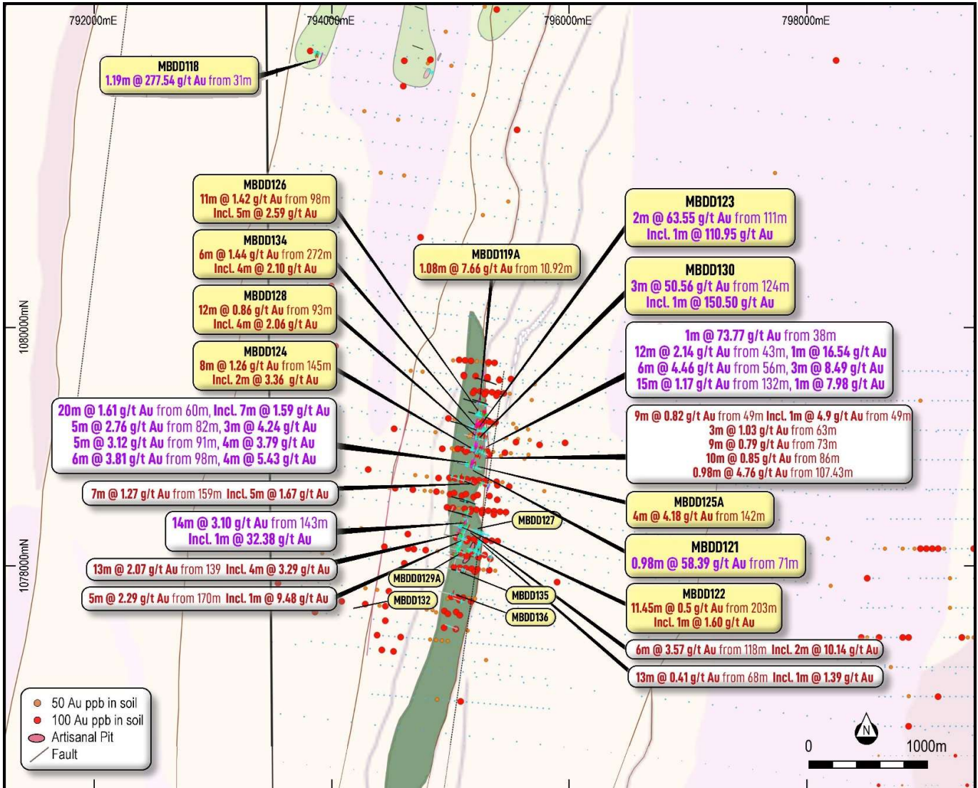
Figure 3: BM tenement plan view showing new significant drilling results (yellow) at BM Target 3
