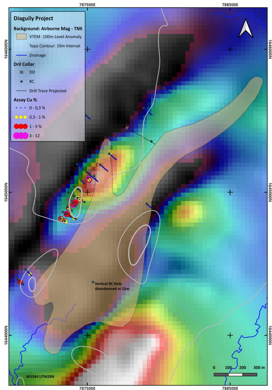
Figure 4 - 100 m VTEM level anomaly (beige polygon) over airborne TMI magnetics, with historical drill collars, projected drill traces and copper assays. Historical drilling lies predominantly west of the modelled conductor. WGS84 UTM Zone 28N. Source: SGC (ASX release 12 October 2026).
