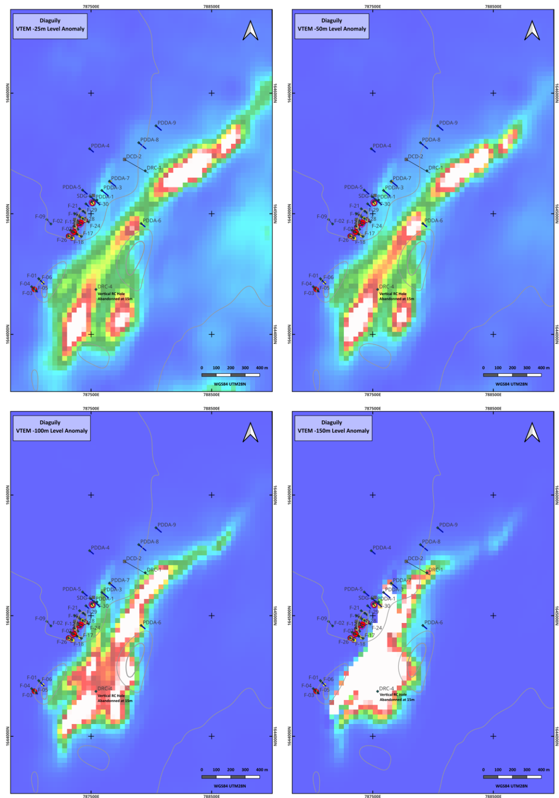
Figure 3 - Reprocessed VTEM conductivity depth slices at 25 m, 50 m (top) and 100 m, 150 m (bottom) below surface, with historical drill collars and projected drill traces. WGS84 UTM Zone 28N. Source: SGC reprocessing of 2008 Shield Mining VTEM data (ASX release 12 October 2026).
