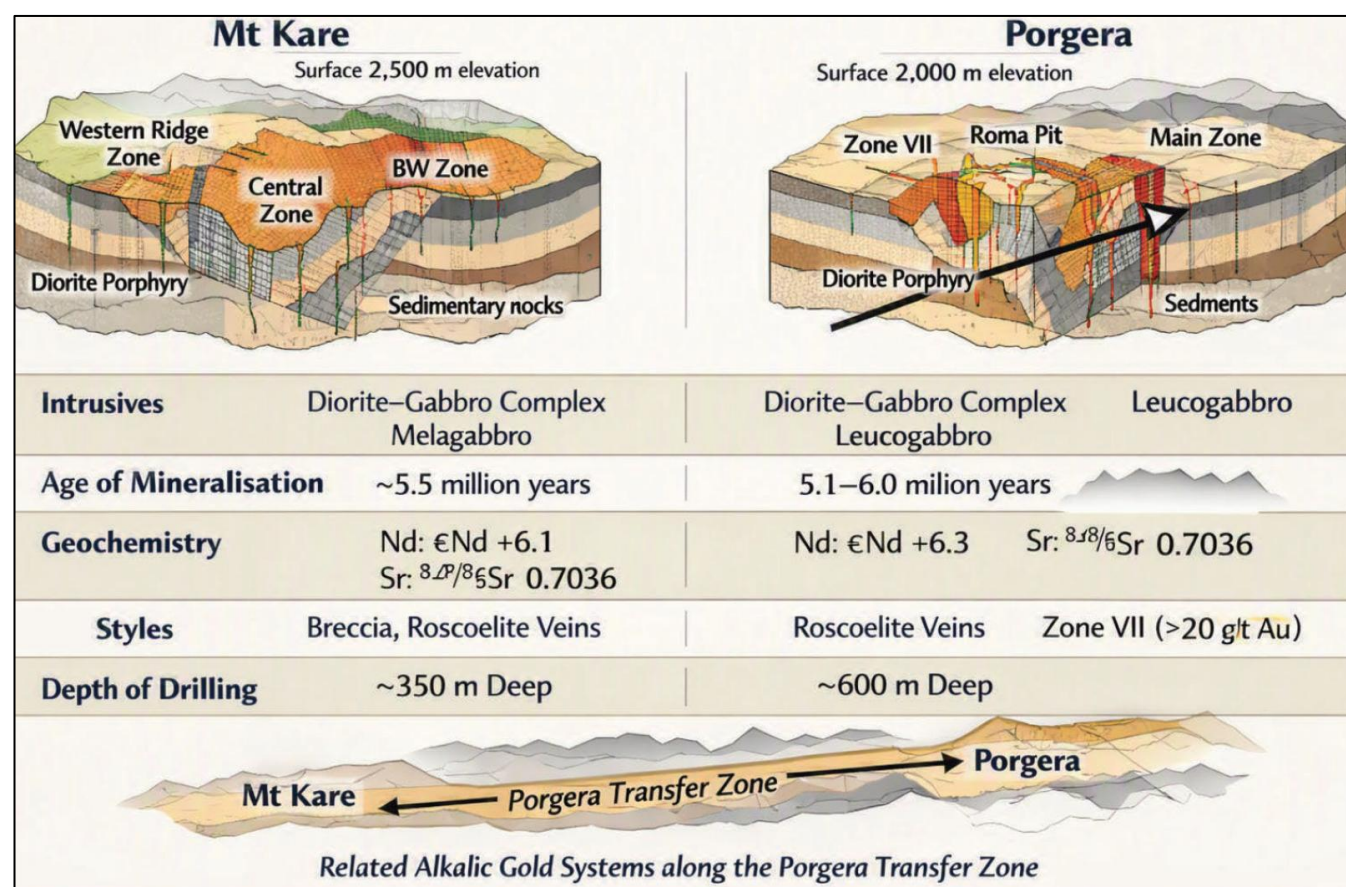
Figure 3: Schematic models of Mt Kare and the nearby Porgera deposit highlighting the greater elevation and potentially less eroded nature of Mt Kare compared to Porgera. Source:after Richards & Ledlie 1993 8 .
