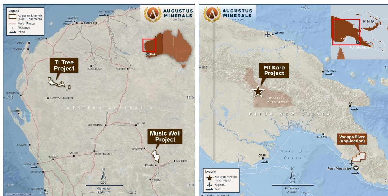
Figure 18 Augustus Minerals Project Locations.
