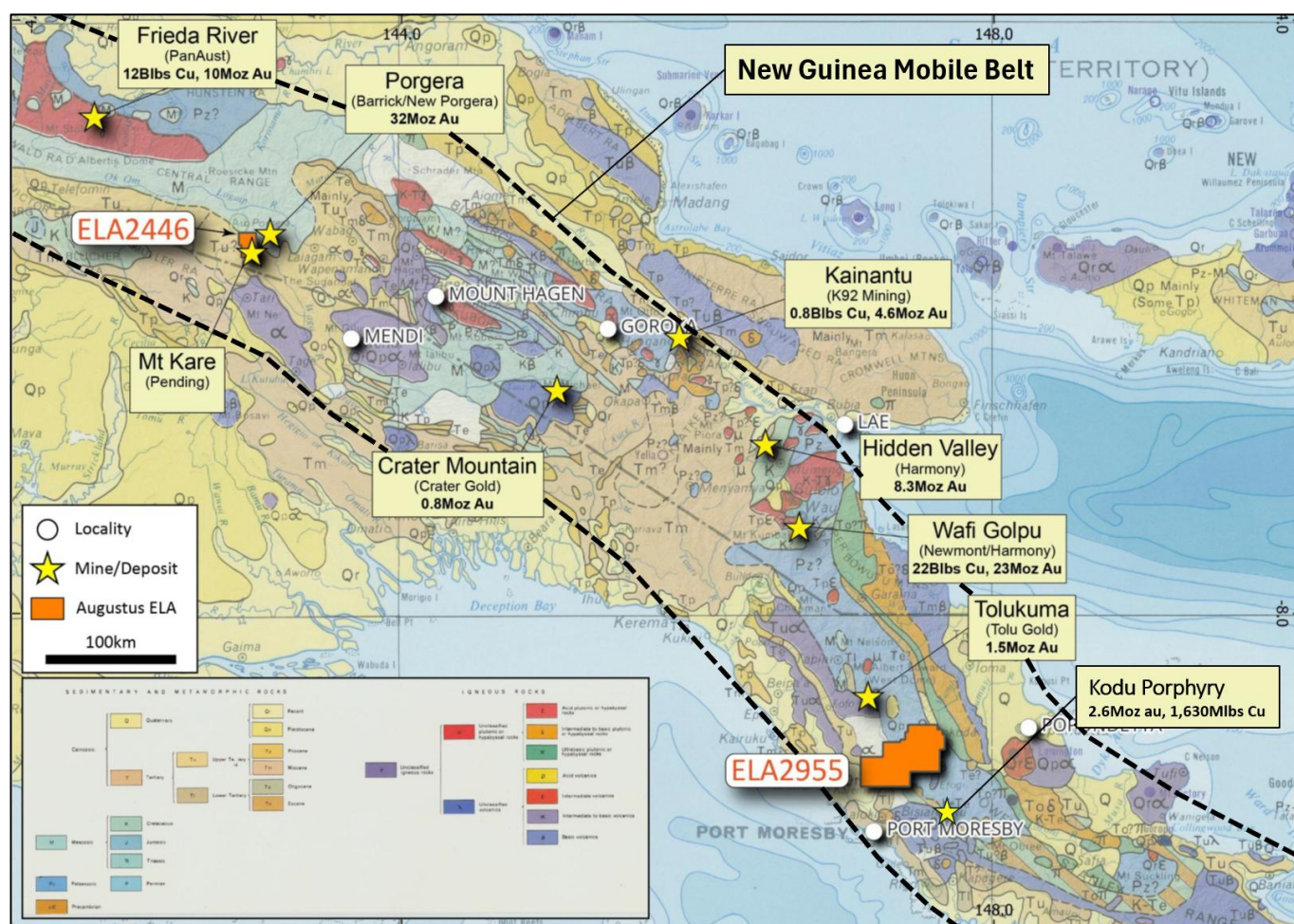
Figure 1: Location of Augustus/ACM PNG Tenement Applications in relation to significant gold & copper deposits (Geological Map of the Territory of Papua and New Guinea, 1963, Australian Bureau of Mineral Resources).
