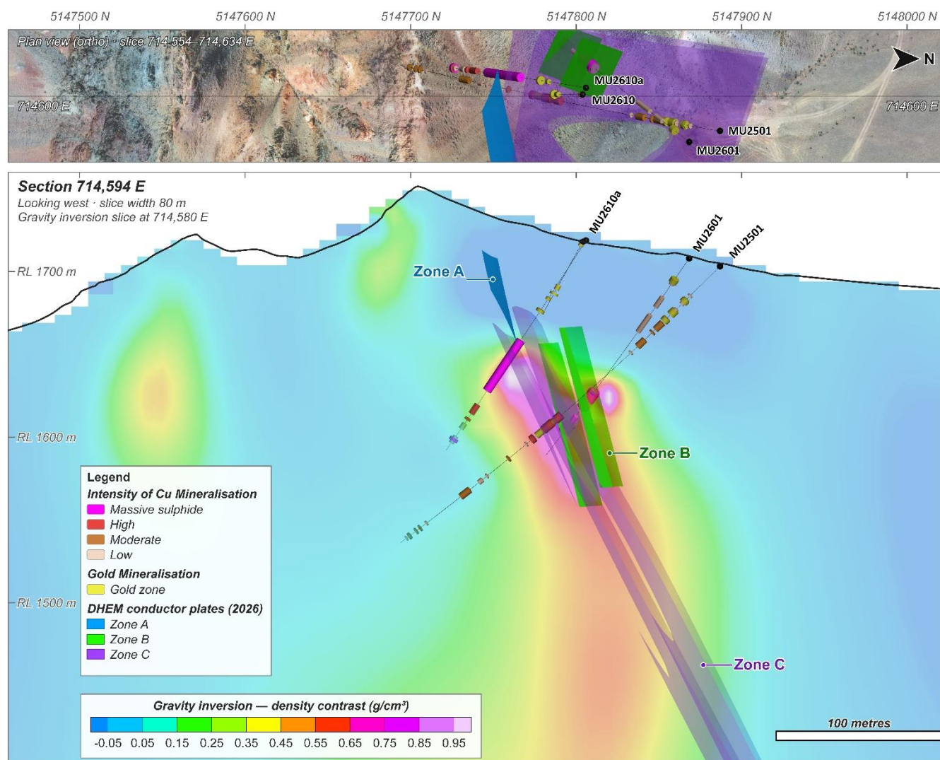
Figure 3. Constrained gravity inversion + new DHEM plates
