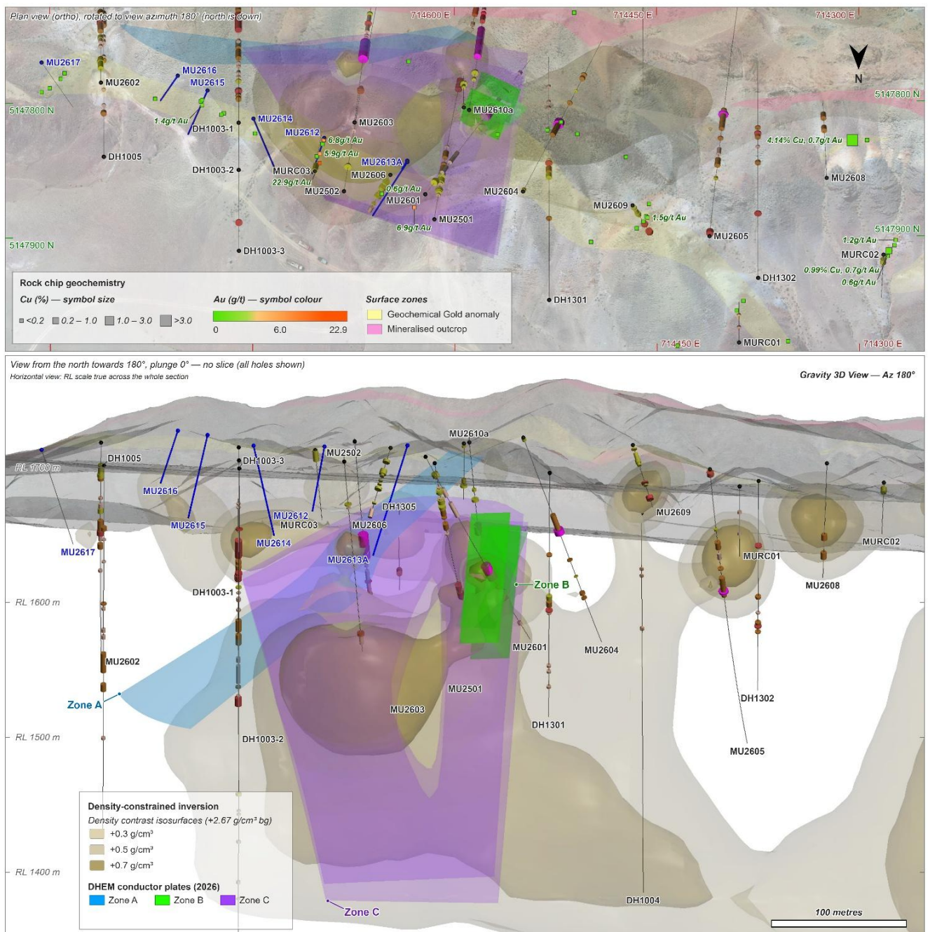
Figure 2. Longitudinal section along with constrained gravity inversion + new DHEM plates.
