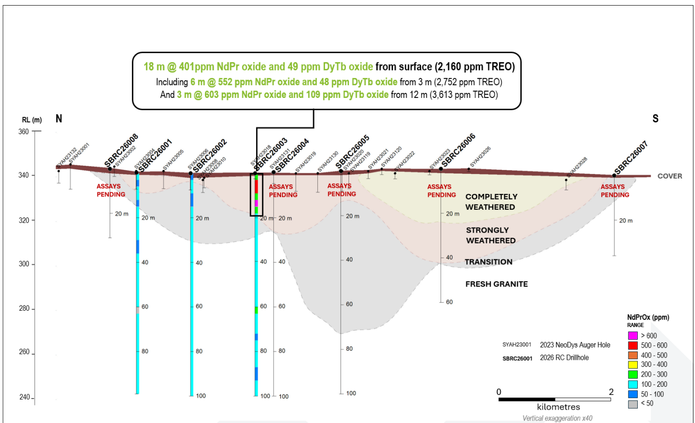
Figure 2 – Cross section interpretation displaying weathering profiles NdPr results along drillhole traces from the 2026 RC drilling program at Newmans. Note assay results for drillholes SBRC26004, SBRC26005, SBRC26006, SBRC26007 and SBRC26008 are still pending.
