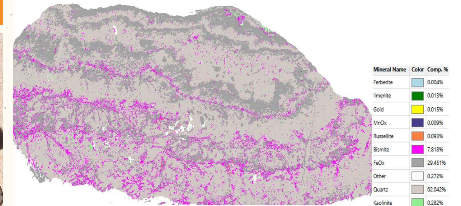
Deconvoluted elemental map and spectra from the Bruker M4 TORNADO PLUS, confirming the presence of Bismuth and Gold (7)
